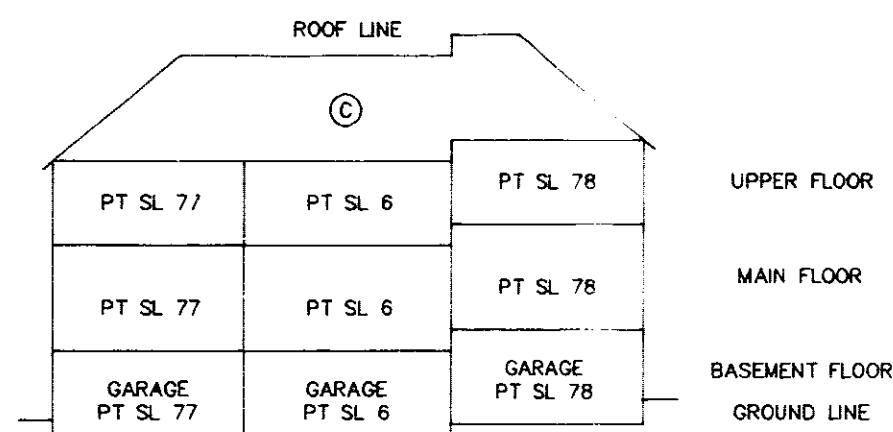
BLOCK 21 : SECTION U-U
