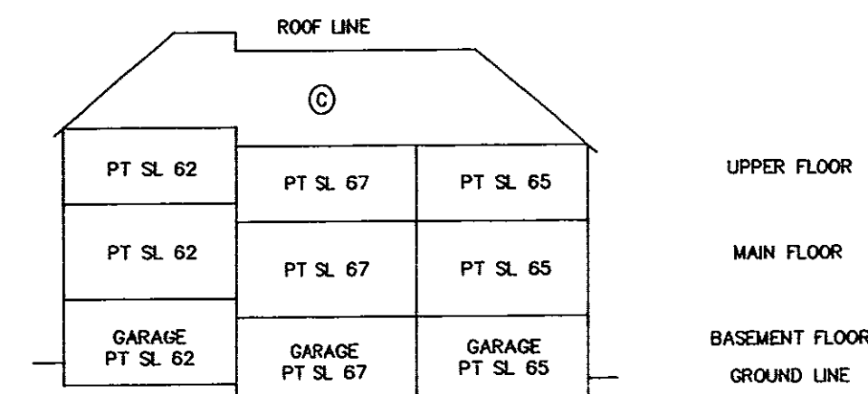
BLOCK 24 : SECTION X-X
