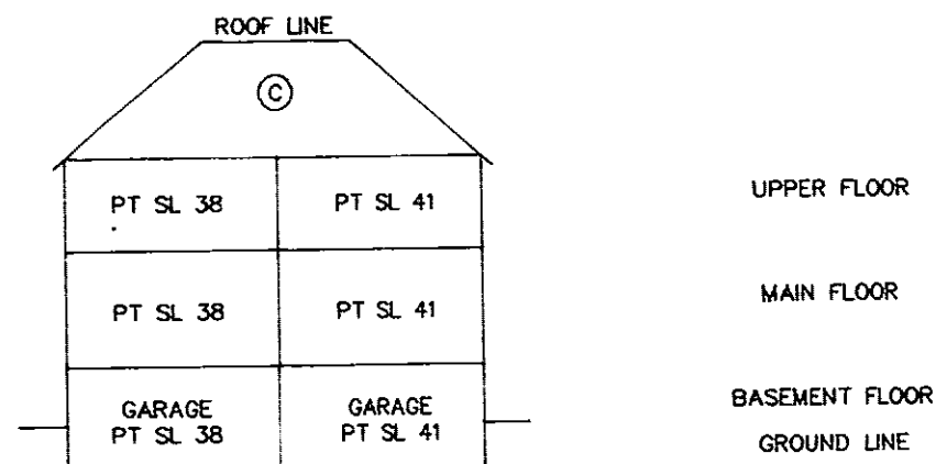
BLOCK 27 : SECTION AA-AA
